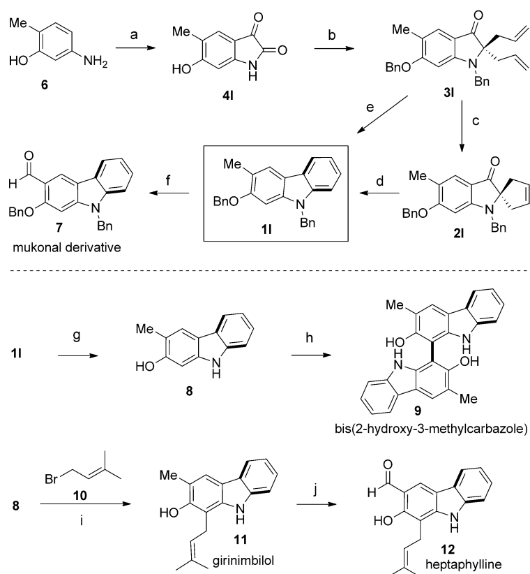
Scheme 8. Synthesis of naturally occurring carbazole alkaloids. a) 1. \text{CCl}_3\text{CH}(\text{OH})_2 , \text{NH}_2\text{OH}\cdot\text{HCl} , \text{Na}_2\text{SO}_4 , 60^\circ\text{C} , 12 h; 2. \text{H}_2\text{SO}_4 , 80^\circ\text{C} , 30 min, 65%; b) 1. \text{BnBr} , \text{K}_2\text{CO}_3 , DMF, room temperature, 8 h, 95%; 2. \text{allylMgBr} , THF, room temperature, 2 h, 75%; c) G-II (5 mol%), \text{CH}_2\text{Cl}_2 , 8 h, room temperature, 88%, or G-I (10 mol%), \text{CH}_2\text{Cl}_2 , 18 h, room temperature, 78%; d) \text{TsOH} (10 mol%), toluene, 80^\circ\text{C} , 3 h, 95%; e) G-II (5 mol%), \text{TsOH} (10 mol%), 80^\circ\text{C} , 6 h, 86%; f) DDQ, MeOH, room temperature, 30 min, 91%; g) 10% Pd/C, \text{H}_2 , MeOH, 36 h, room temperature, 98%; h) \text{CuCl}_2 (10 mol%), DBU, MeCN, 100^\circ\text{C} , 26 h, 51%; i) 10 , DIPEA, \text{CH}_2\text{Cl}_2 , 12 h, room temperature, 67%; j) DDQ, MeOH, room temperature, 30 min, 85%. DBU = 1,8-diazabicyclo[5.4.0]undec-7-ene, DDQ = 2,3-dichloro-5,6-dicyano-1,4-benzoquinone, DIPEA = N,N -diisopropylethylamine.
