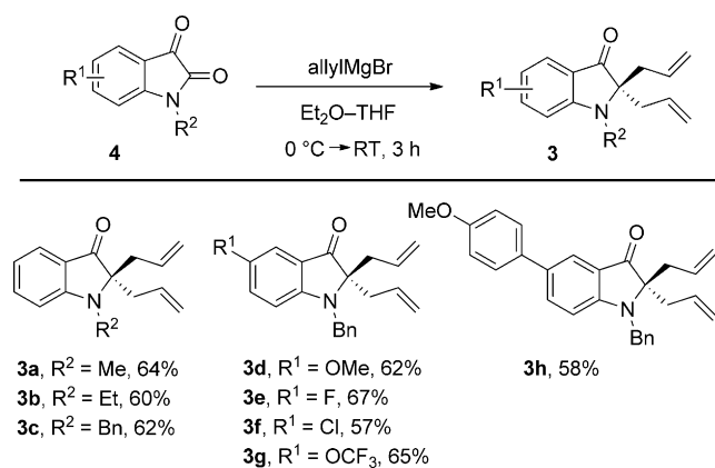
Scheme 2. Exploration of the allyl Grignard addition to isatin derivatives. Reaction conditions: 4 (2.0 mmol, 1.0 equiv), allylmagnesium bromide solution (1 M in Et 2 O, 5.0 equiv), Et 2 O–THF (10 mL), room temperature, 3 h. Bn = benzyl.
