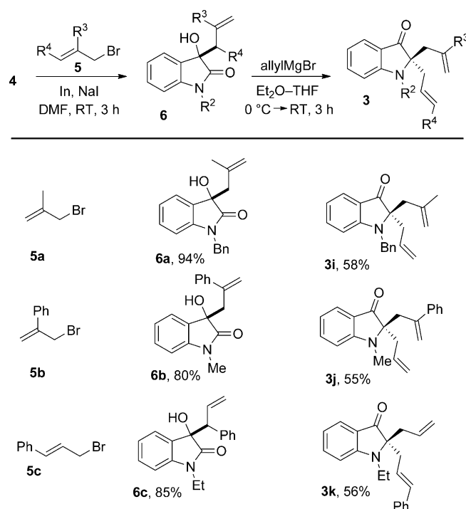
Scheme 4. Sequential addition of allylindium [a] and Grignard reagents [b] to isatin derivatives. [a] Reaction conditions: 4 (2.0 mmol, 1.0 equiv), allyl bromide (1.6 mmol), NaI (1.6 mmol), indium metal (1 mmol), DMF, room temperature. [b] Reaction conditions: 6 (2.0 mmol, 1.0 equiv), allylmagnesium bromide solution (1 M in Et 2 O, 3.0 equiv), Et 2 O–THF (10 mL), room temperature, 3 h. DMF = N,N -dimethylformamide.
