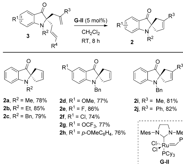
Scheme 5. Ring-closing metathesis of diallyl 3-oxindole derivatives. Reaction conditions: 3 (0.3 mmol, 1.0 equiv), G-II catalyst (5 mol %), CH 2 Cl 2 (4 mL), room temperature, 8 h. Cy = cyclohexyl, Mes = 2,4,6-trimethylphenyl.
