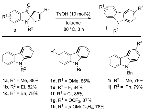
Scheme 6. One-pot ring rearrangement-aromatization (RRA) of spirocyclic 3-oxindoles to carbazoles. Reaction conditions: 2 (0.2 mmol, 1.0 equiv), TsOH (10 mol %), toluene (5 mL), 80 °C, 3 h.
