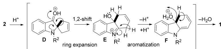
Scheme 7. Proposed mechanism for the aromatization-driven ring rearrangement.
