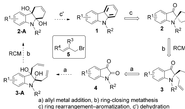
Scheme 1. A general approach to carbazoles.
