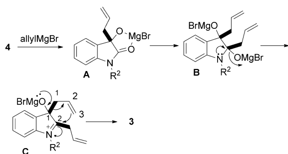
Scheme 3. Proposed rearrangement pathway for the formation of 2,2-diallyl 3-oxindoles 3 .
